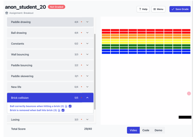
Figure 3: The user interface for our grading tool.
